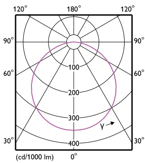
Downlight DN016B CW 15W D125 RD ND-LDD
